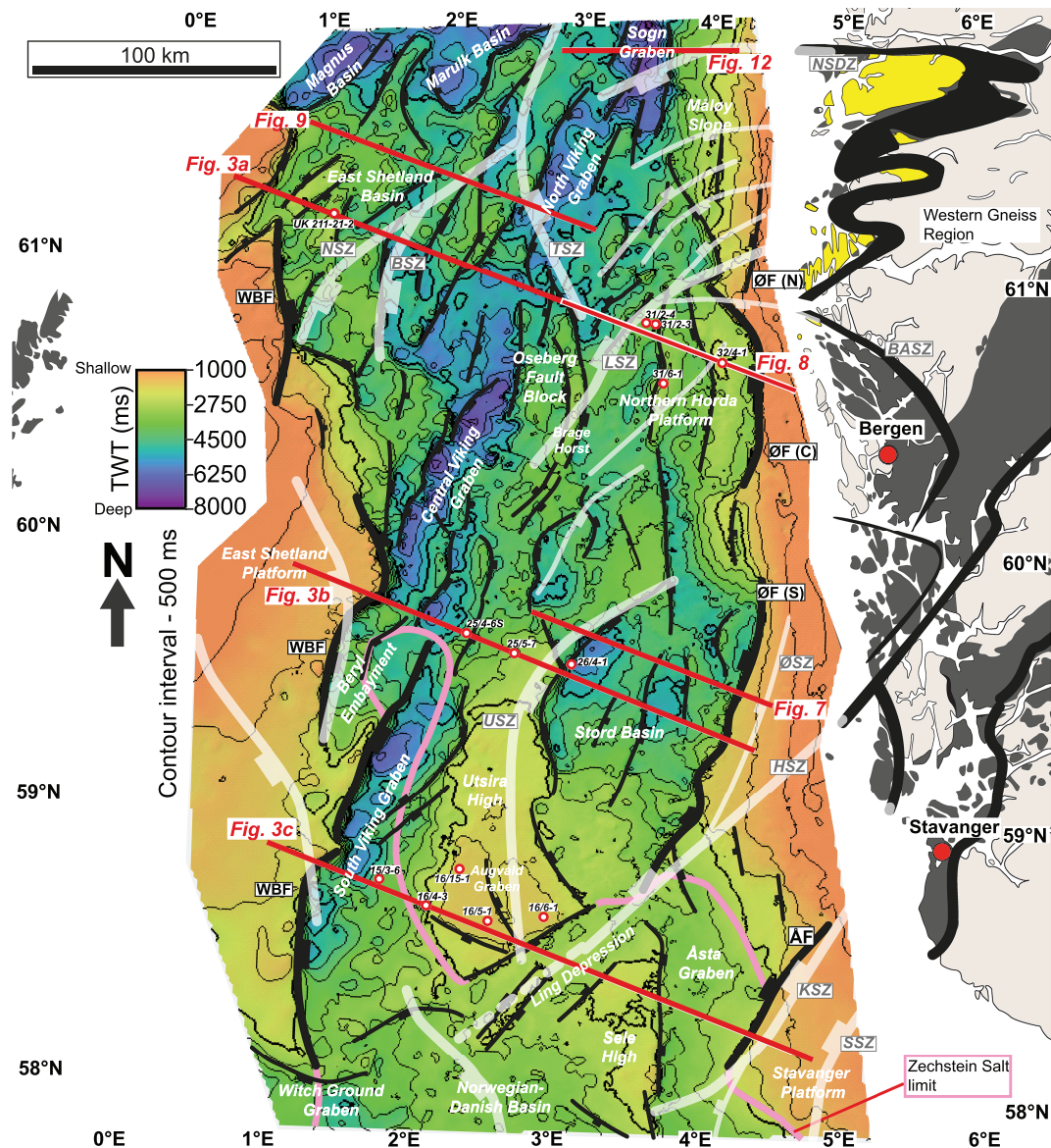
Figure 4. Two-way-time (TWT) structure map of the Base RP1 structure map, modified after Fazlikhani et al. (2017). See Figures 2 and 3 for structural level. The offshore extensions of Devonian shear zones are shown by white translucent lines (after Fazlikhani et al., 2017), with those referred to in the study labeled in gray. The Utsira High forms an intrabasinal high in the south of the area. The pink line represents the northern limit of mobile salt of the Zechstein Supergroup. Major structural lows include the Stord Basin, East Shetland Basin, and the Viking Graben and Sogn Graben. Faults: WBF = Western Boundary Fault, ØF (S/C/N) = Øygarden Fault (South/Central/North), ÅF = Åsta Fault. Shear Zones: NSZ = Ninian Shear Zone, BSZ = Brent Shear Zone, TSZ = Tampen Shear Zone, LSZ = Lomre Shear Zone, USZ = Utsira Shear Zone, HSZ = Hardangerfjord Shear Zone, KSZ = Karmøy Shear Zone, SSZ = Stavanger Shear Zone.
